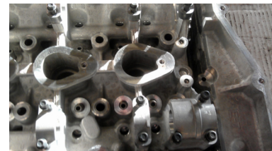
Diesel engine head after being emersed in Enviro-Green MAX for fifteen minutes at ambient temperature.
