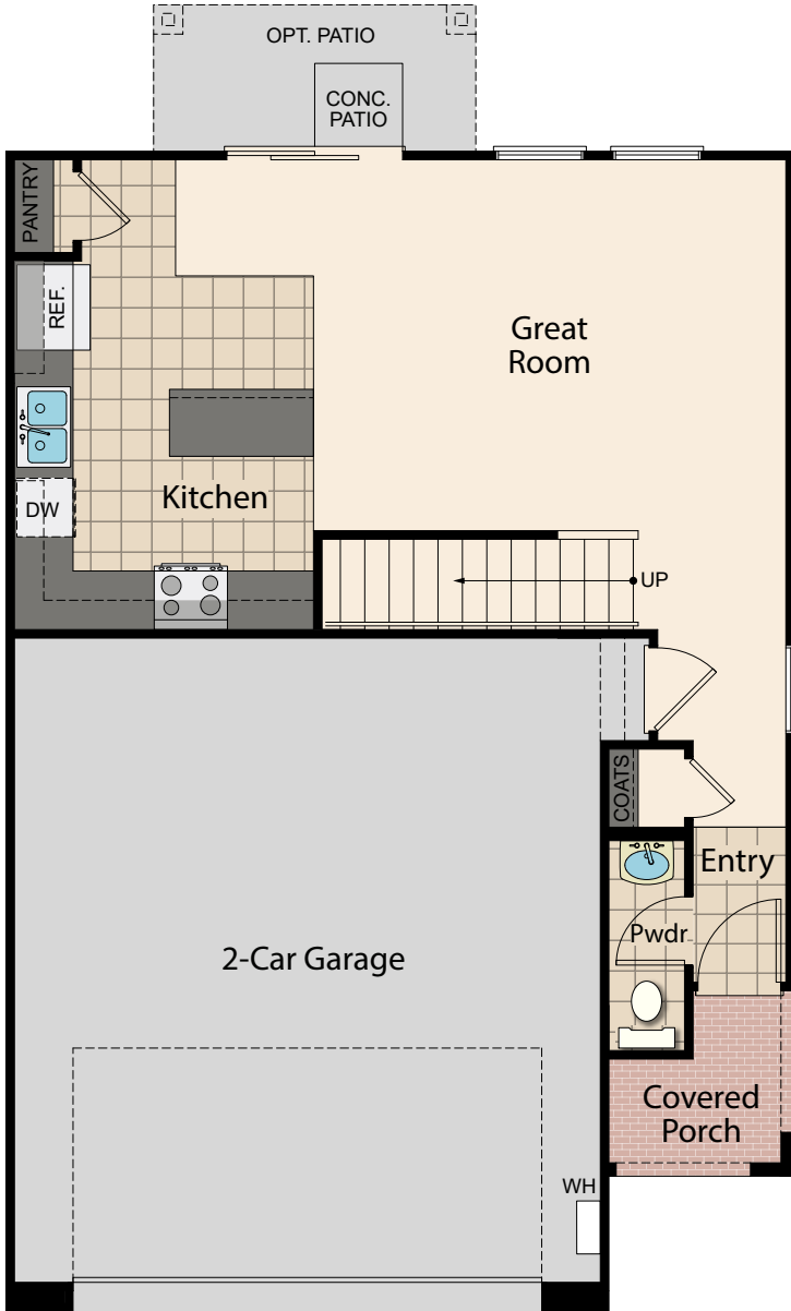
First Floor
