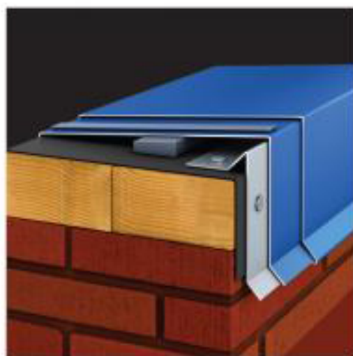
Standard Coping
