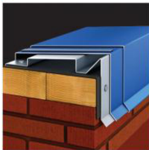
Spring-Tite Coping
