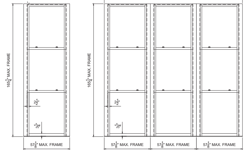
TRIPLE-HUNG SASH WEIGHT AND CHAIN WINDOWS
