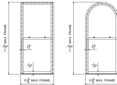
DOUBLE-HUNG BALANCE WINDOWS
