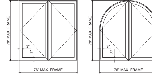
INSWING/OUTSWING TWIN CASEMENT WINDOWS
