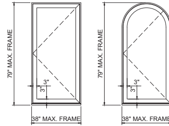
OUTSWING SINGLE CASEMENT WINDOWS
