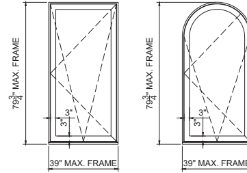
INSWING/TILT&TURN SINGLE CASEMENT WINDOWS
