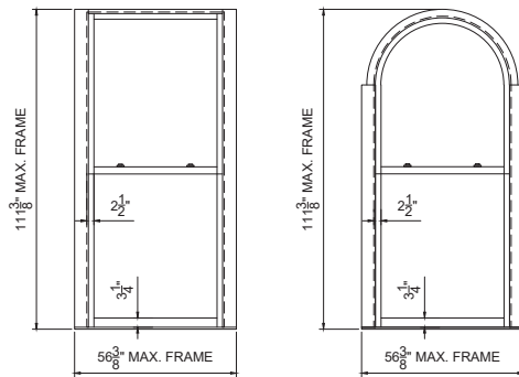
DOUBLE-HUNG SASH WEIGHT AND CHAIN WINDOWS
