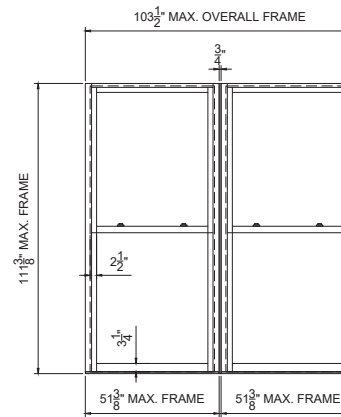
TWIN DOUBLE-HUNG BALANCE WINDOWS
