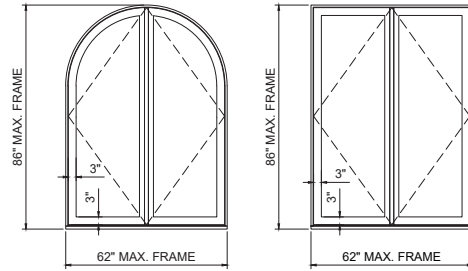
INSWING/OUTSWING FRENCH CASEMENT WINDOWS
