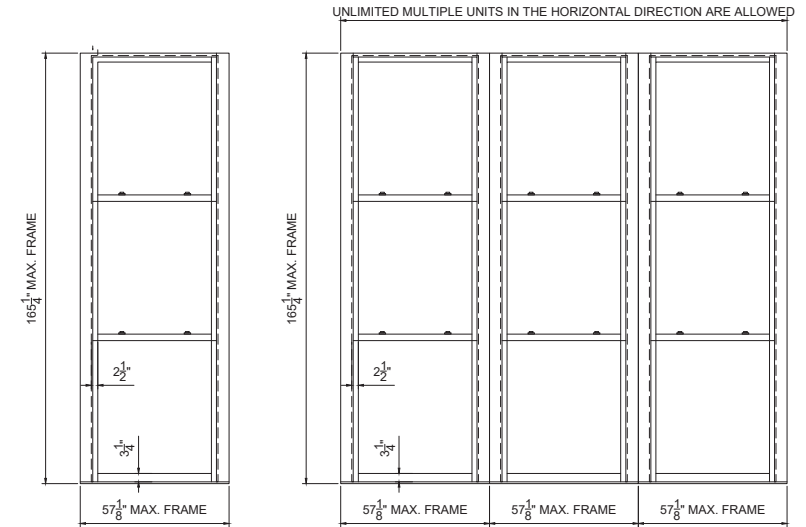
TRIPLE-HUNG SASH WEIGHT AND CHAIN WINDOWS
