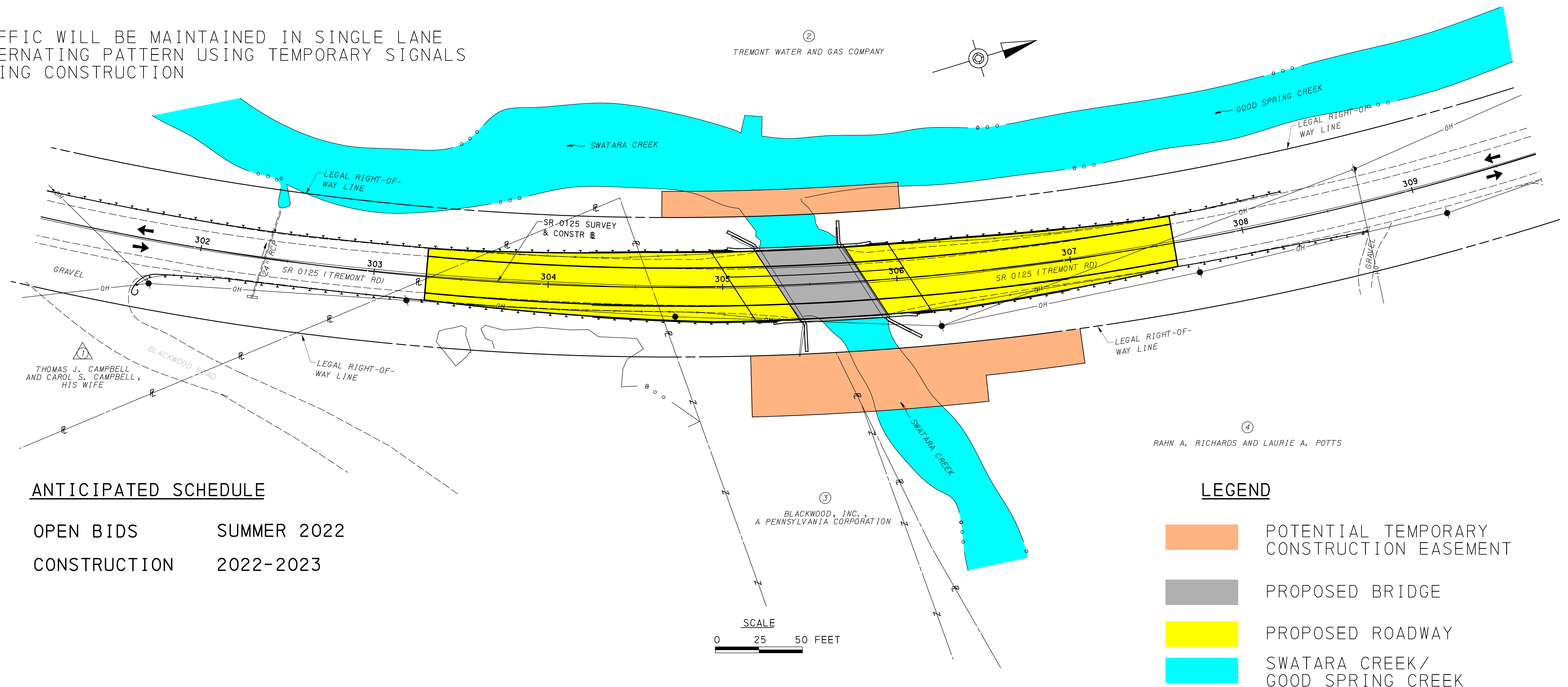
STAGE 1 CONSTRUCTION
