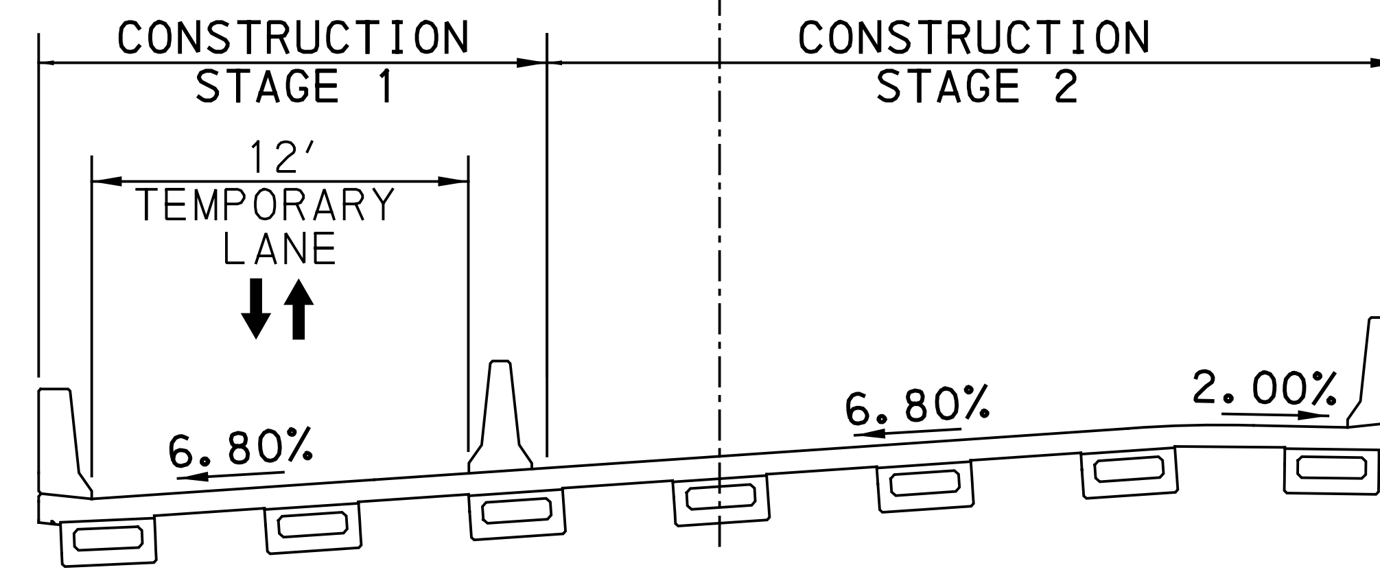
STAGE 2 CONSTRUCTION
