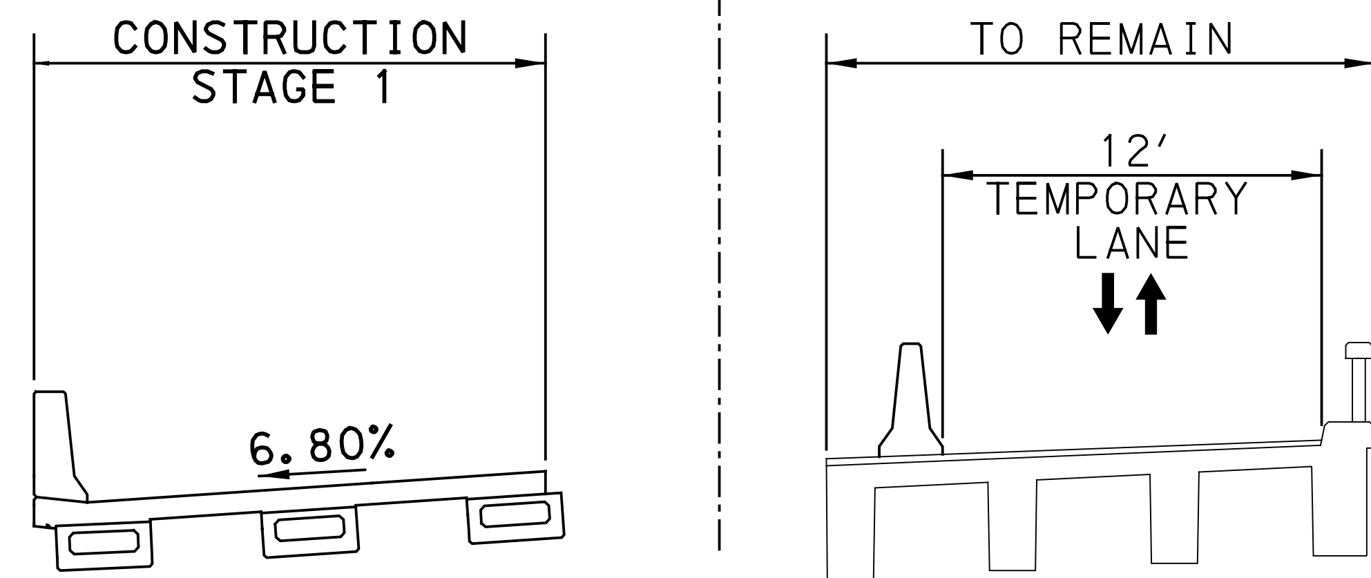
STAGE 1 CONSTRUCTION
