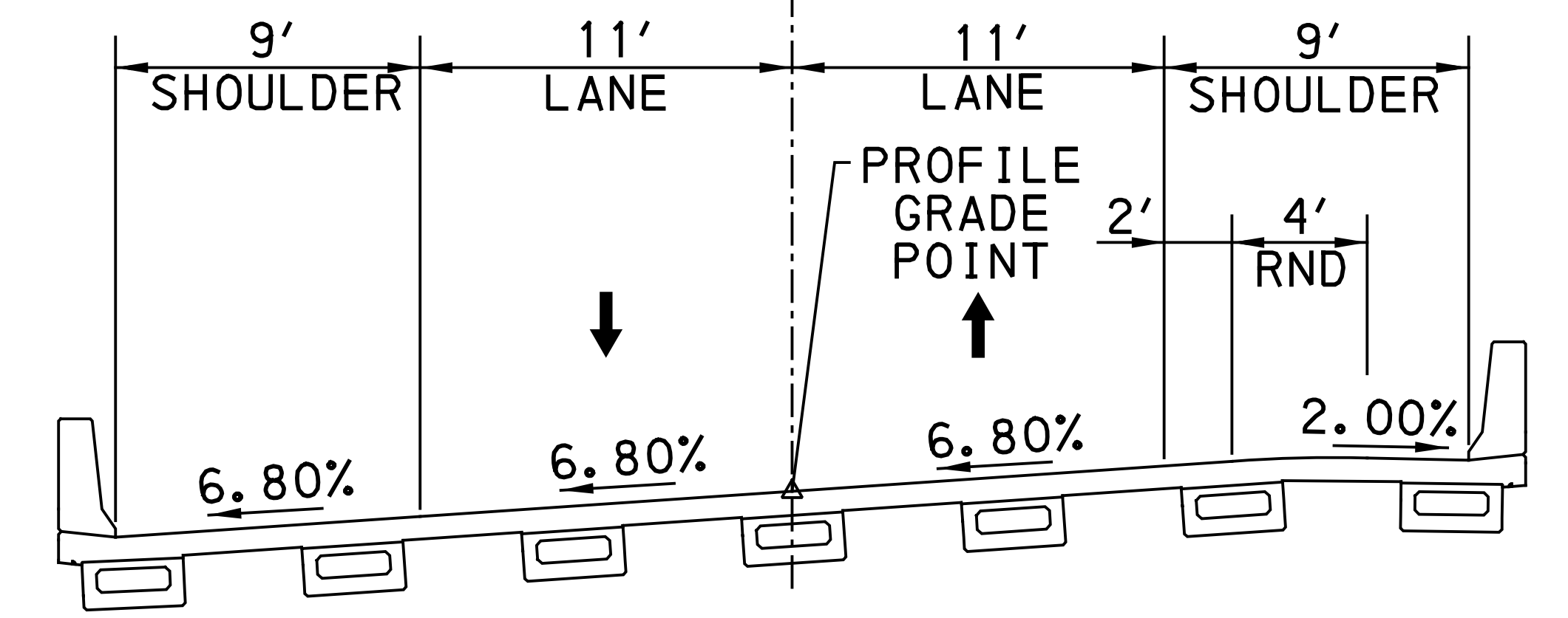
SR 0125 NORMAL SECTION (STRUCTURE)
