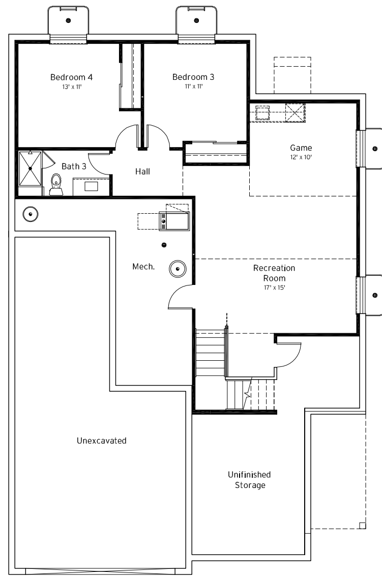
Opt. Finished Lower Level Floor Plan
