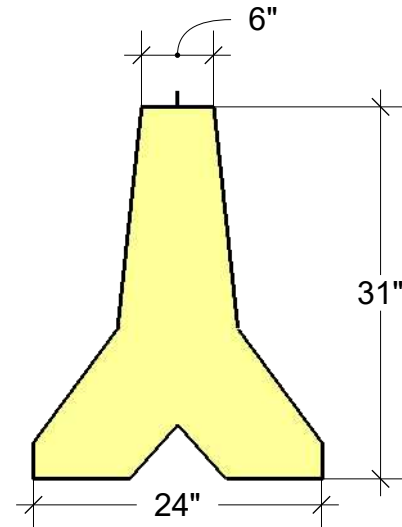
Right Side View Scale: 3/4"=1'-0"
