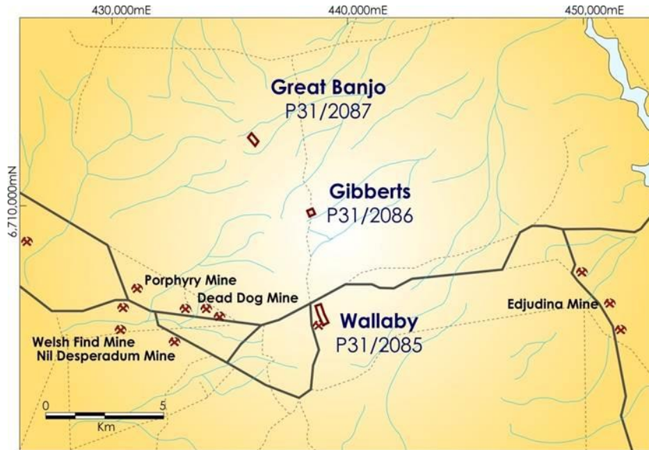
Figure 2 – Yarrie Project - Prospect Locations
