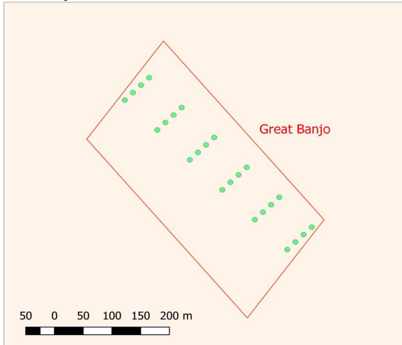
Figure 5 – Great Banjo - Planned Drill Holes
