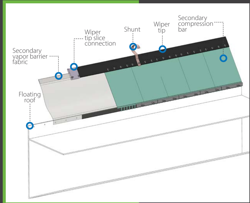
DT-S1 Secondary Metallic Wiper Seal
