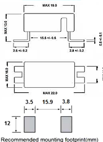
Recommended mounting footprint(mm)
