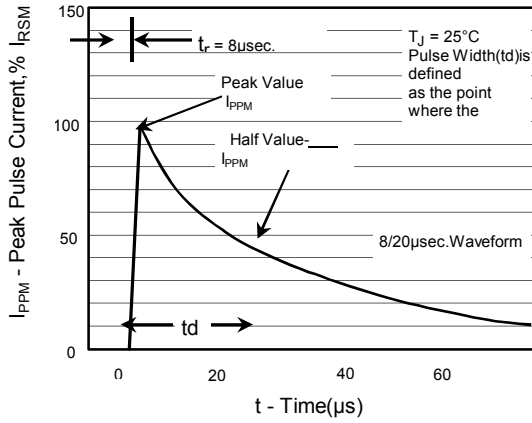
Fig.1 - Test Pulse
