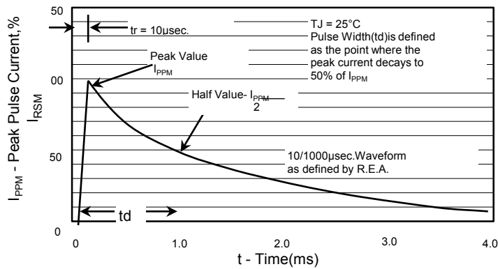
Fig.3 - Pulse Waveform
