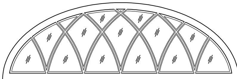
Custom 16 elliptical transom with wooden muntins
