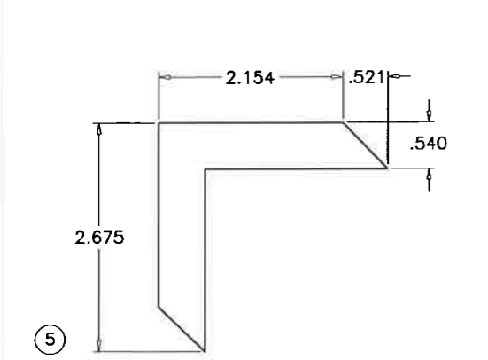
CORNER KEYS
