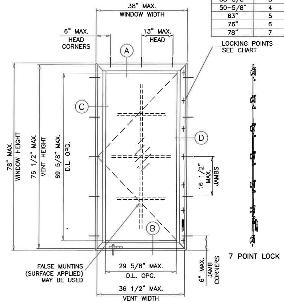
TYPICAL ELEVATION
