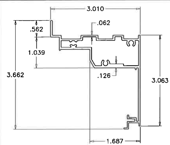
① FRAME
