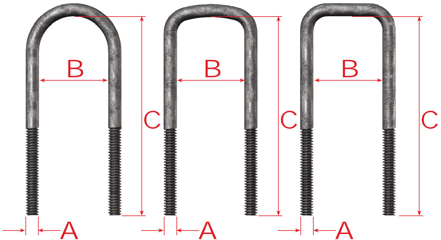
Type 2 Semi-Round Special bend
