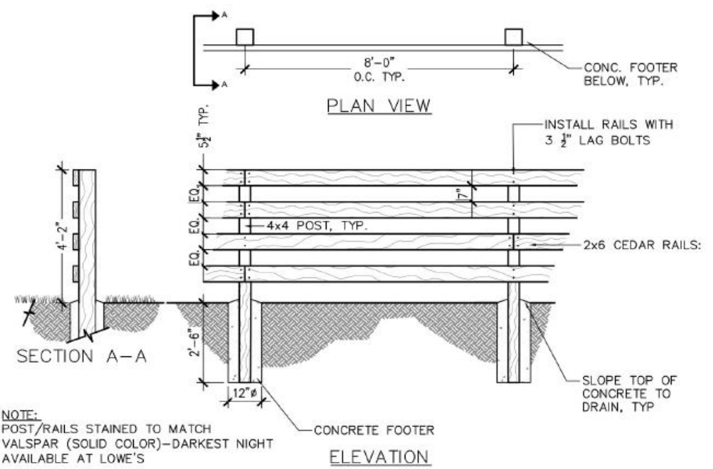
CEDAR 4-RAIL FENCE
