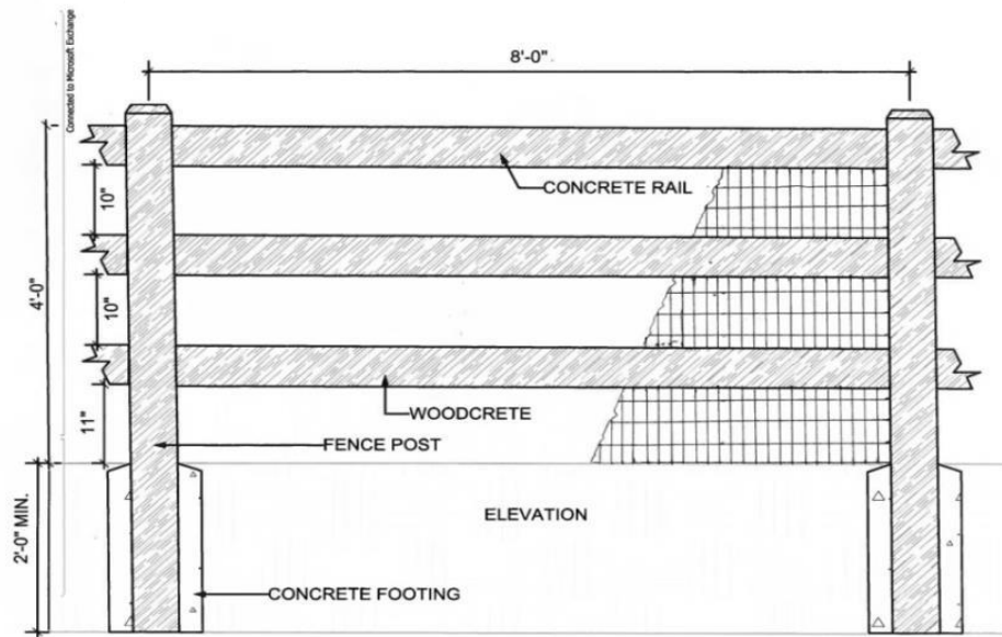
CONCRETE 3-RAIL FENCE
