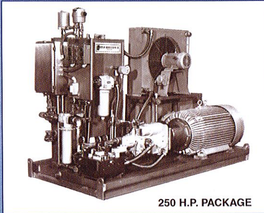
MULTIPLE PUMP PACKAGE
