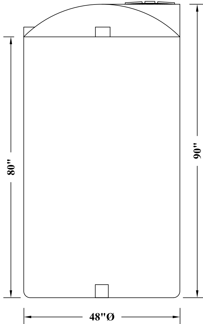
ELEVATION VIEWS
