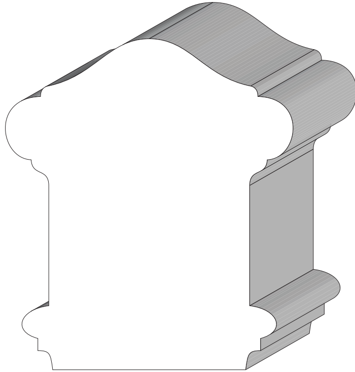
BA 1639 & Cope 3-7/16" x 3"
