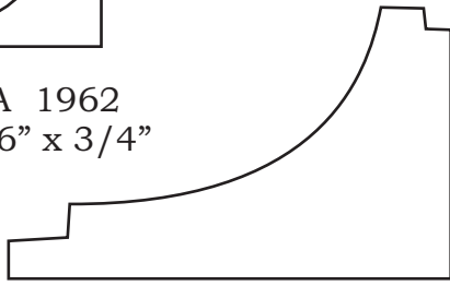
BA 1963 1-5/16" x 2-1/8"
