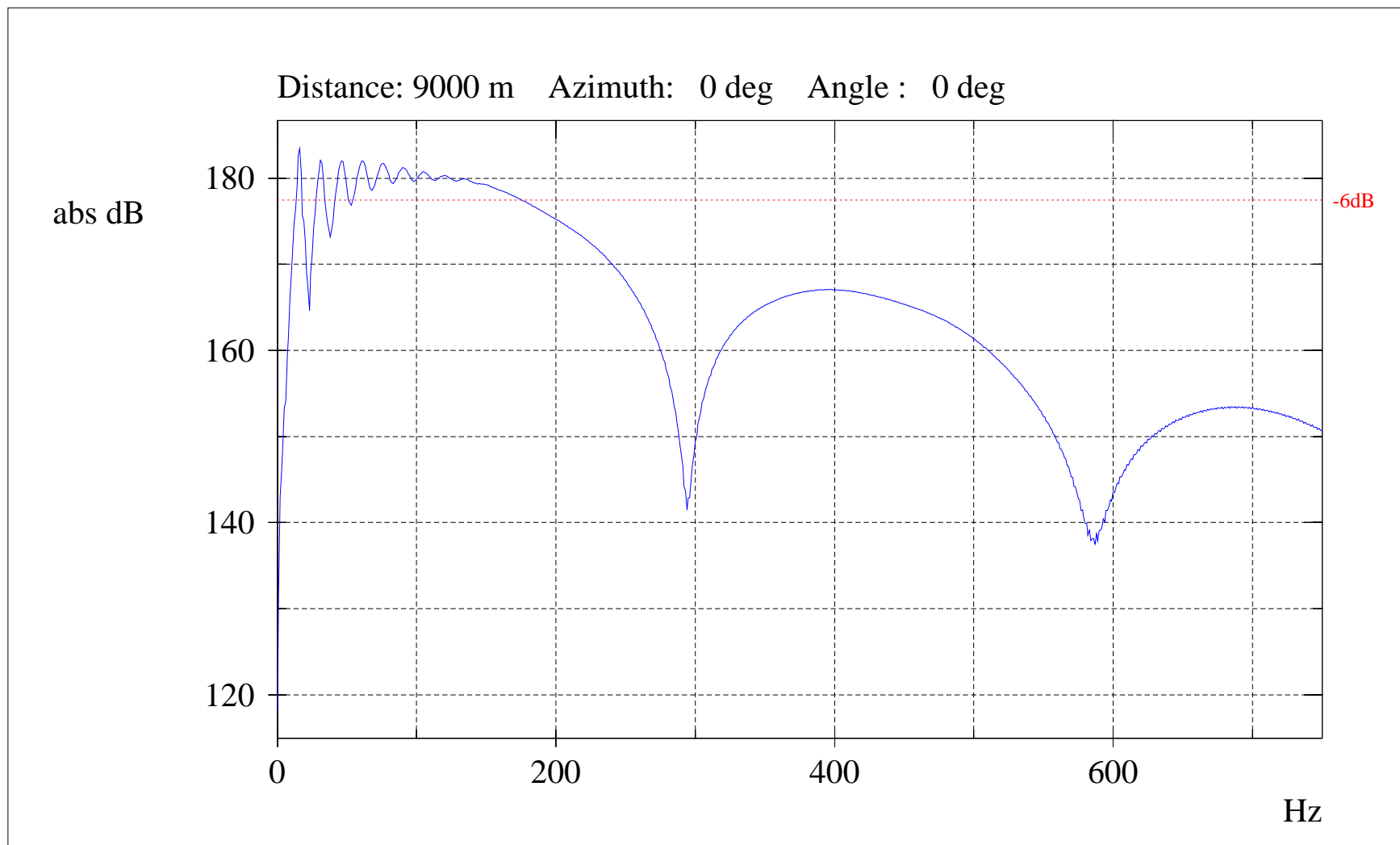
Amplitude spectrum of far-field signature of array : 4x10_2-5m
