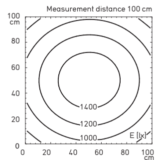
Illuminance based on the example of 62 W with Light Forming Technology
