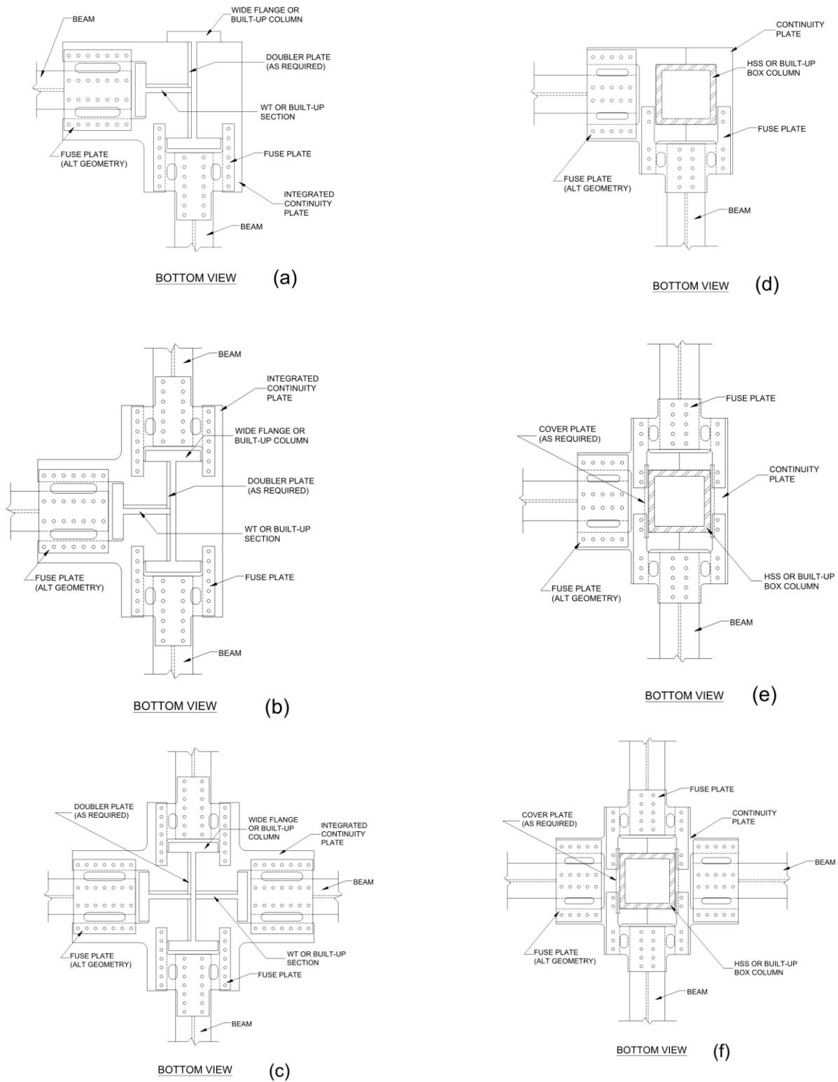
FIGURE 2 – DURAFUSE FRAMES BI-AXIAL CONFIGURATIONS
