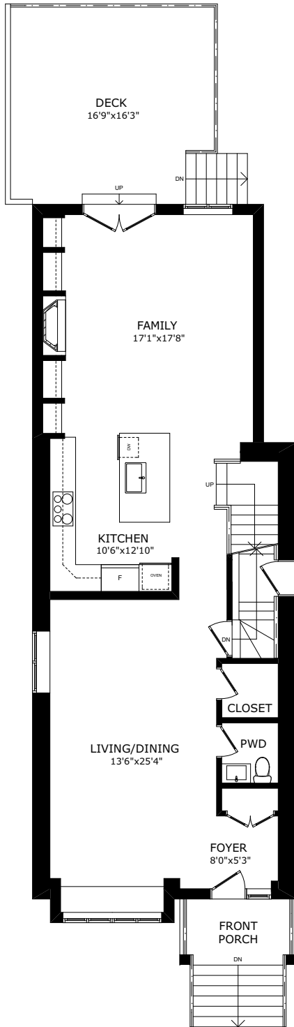
MAIN FLOOR
