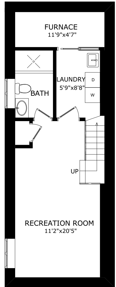
LOWER FLOOR CLG:8'2"
