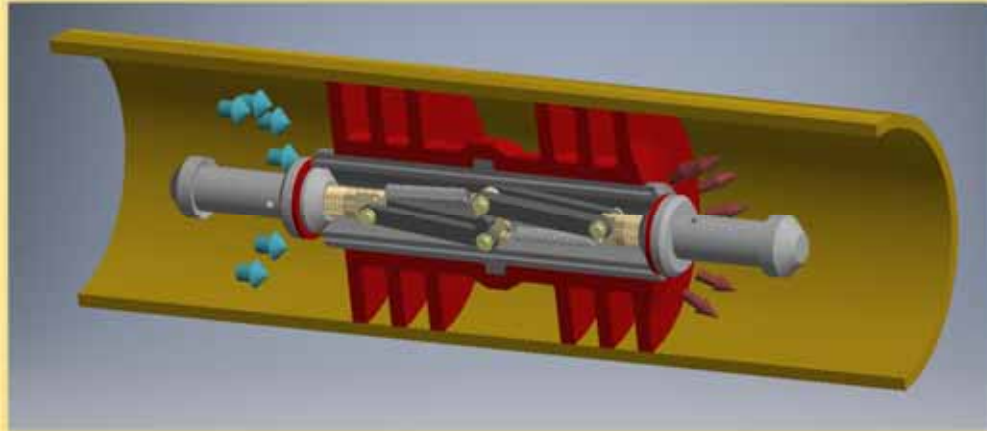
RETRIEVABLE JET PIG
