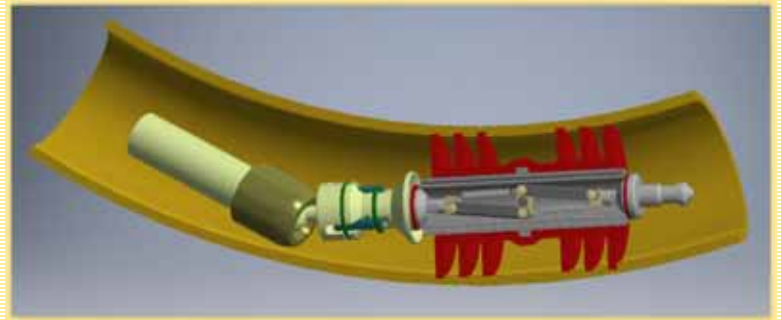
BEING RETRIEVED AROUND A 5D BEND
