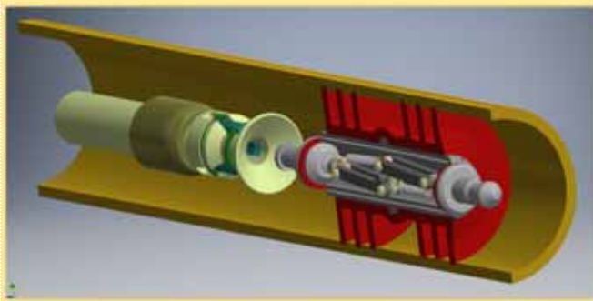
SHOWING A BETA LATCH APPROACHING
