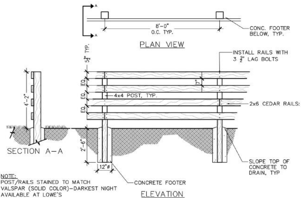
CEDAR 4-RAIL FENCE
