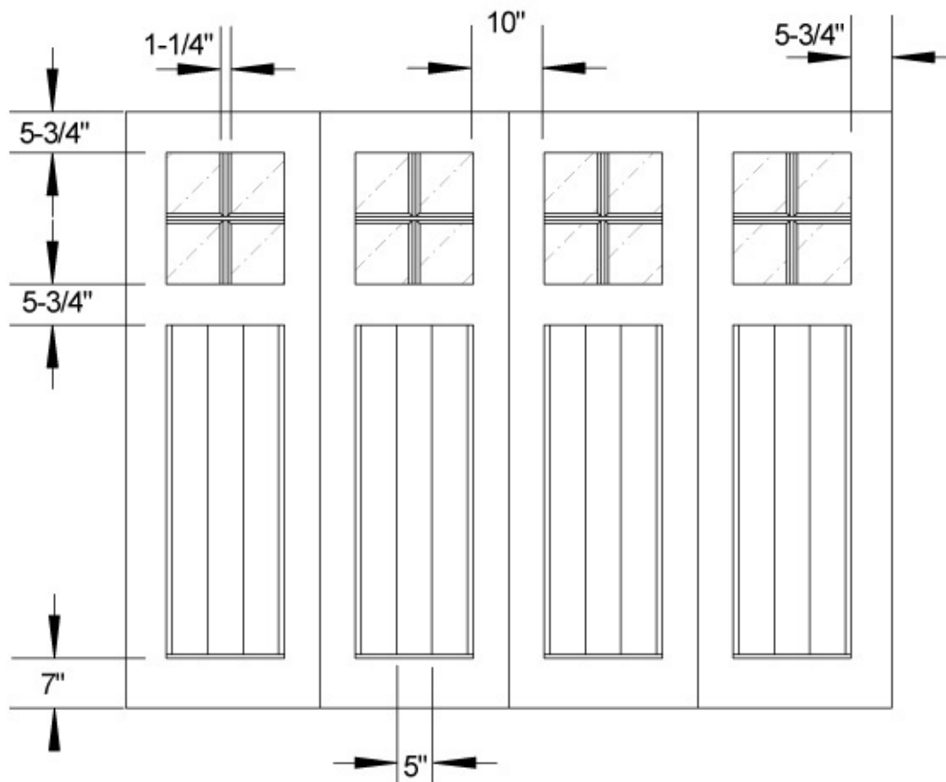
Model BF-16L-4VP Front Elevation Scale: 1/2" = 1'0"
