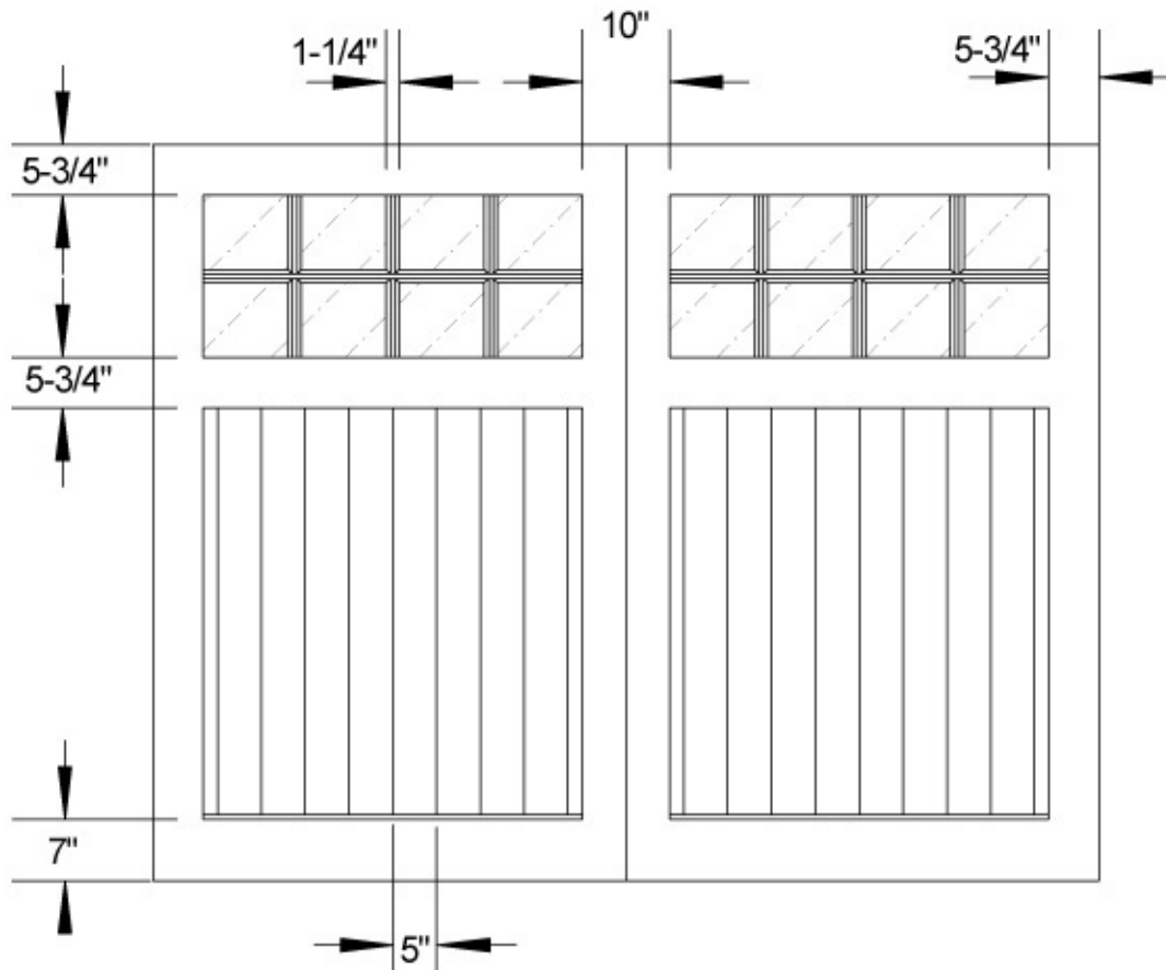
Model 16L-2VP Front Elevation Scale: 1/2" = 1'0"
