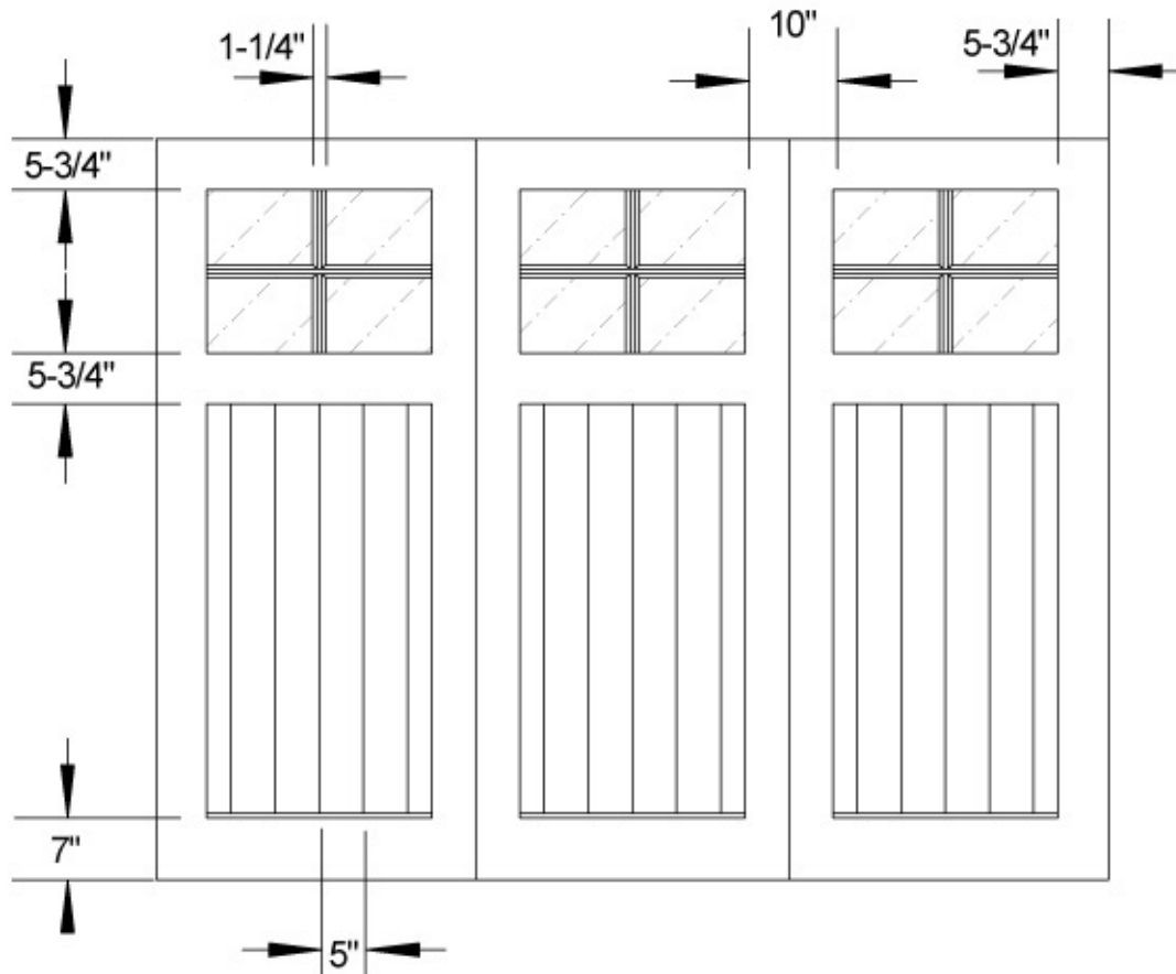
Model TF-12L-3VP Front Elevation Scale: 1/2" = 1'0"
