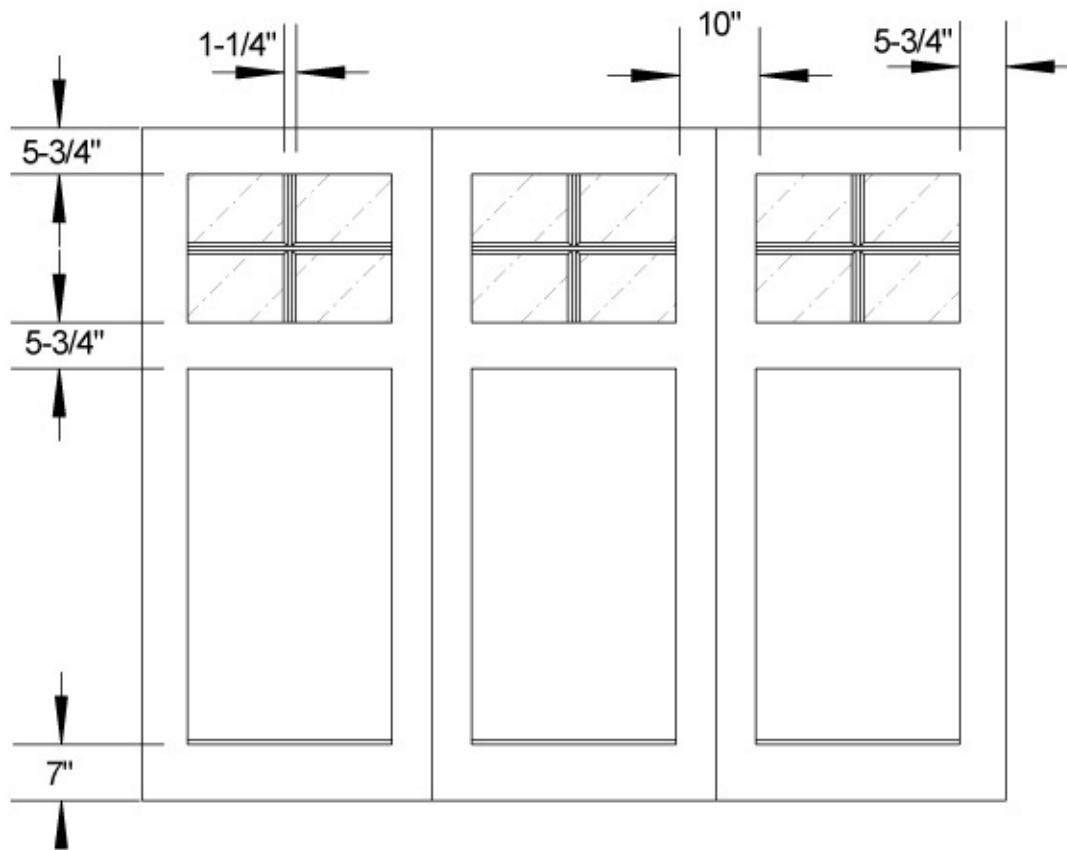
Model TF-12L-3FP Front Elevation Scale: 1/2" = 1'0"
