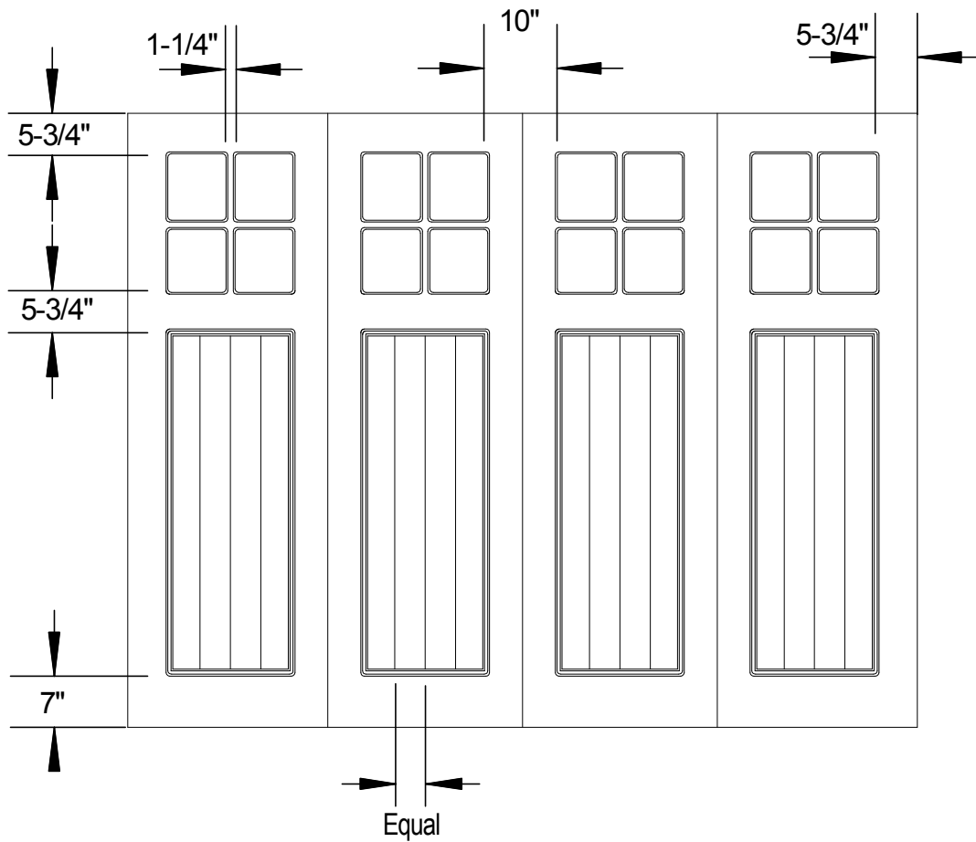
Model BF-16L-4VP Front Elevation Scale: 1/2" = 1'0"
