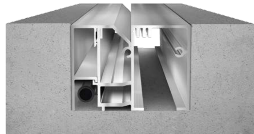
Fully Recessed
