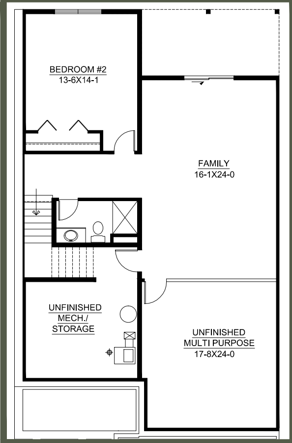
LOWER LEVEL 812 finished sq. ft.
