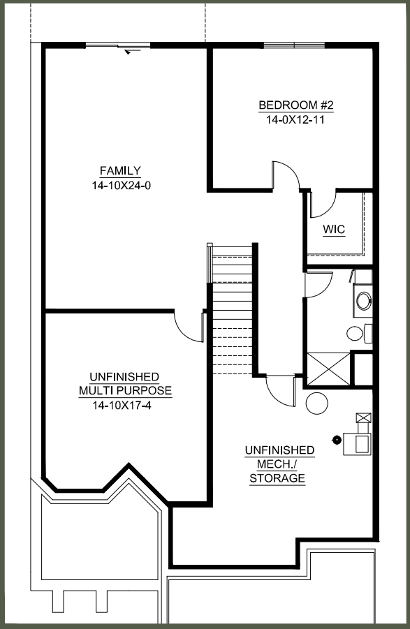
LOWER LEVEL 821 finished sq. ft.
