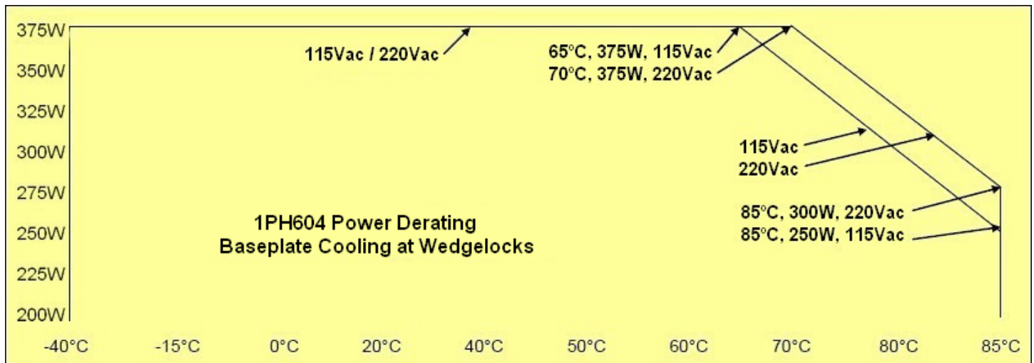
Figure 1: 1PH604 Power De-rating for Temperature and Input Voltage per below graph
