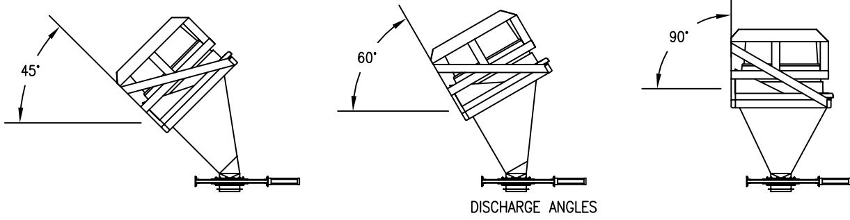
OPEN DISCHARGE UNIT
