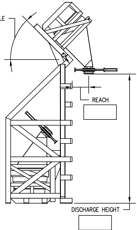
DUST TIGHT, LIFT & DUMP UNIT
