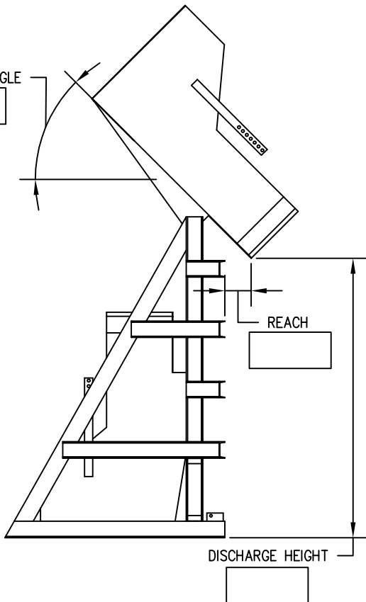
OPEN DISCHARGE, LIFT & DUMP UNIT
