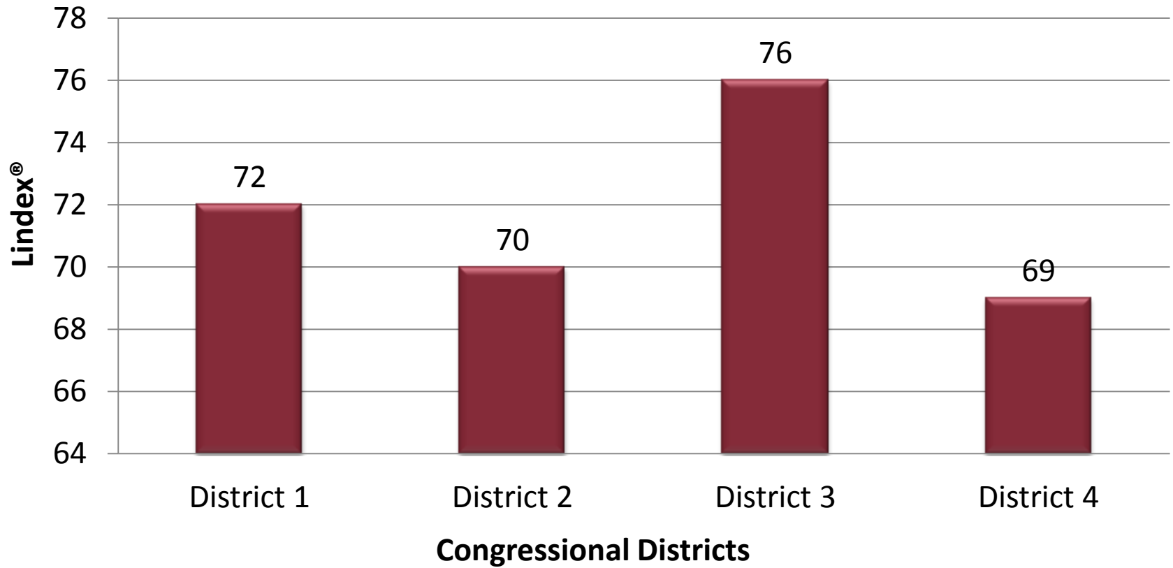
Average of Lindex®
