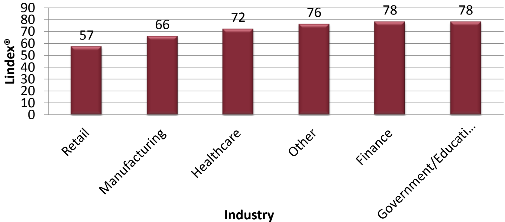
Average of Lindex®
