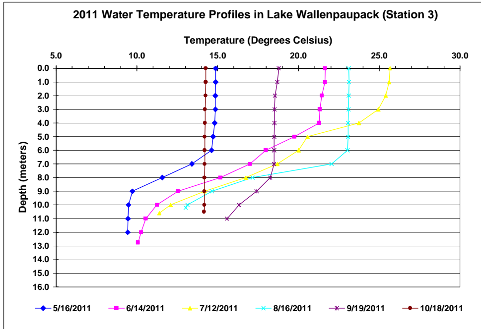
Figure 4.1 Water Temperature Profiles at Station 3 in 2011
