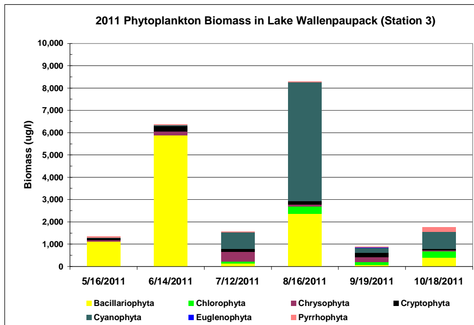
Figure 4.3 Phytoplankton Biomass at Station 3 in 2011
