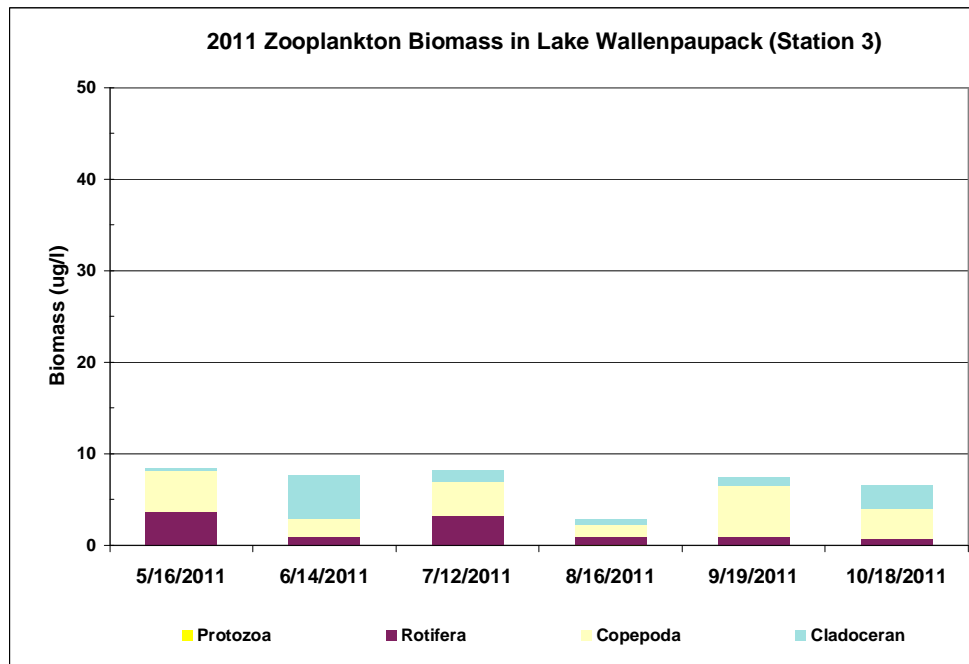
Figure 4.4 Zooplankton Biomass at Station 3 in 2011
