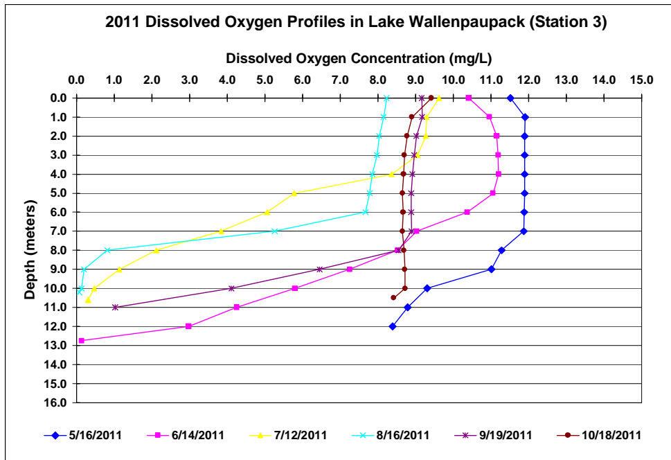
Figure 4.2 Dissolved Oxygen Profiles at Station 3 in 2011
