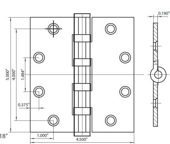
5.0" x 4.5" x SQ
