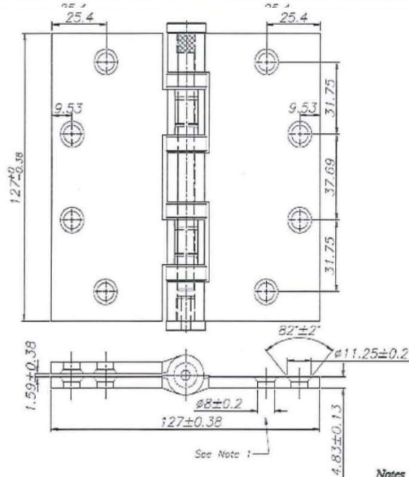
5.0" x 5.0" x SQ (127mm x 127mm)
