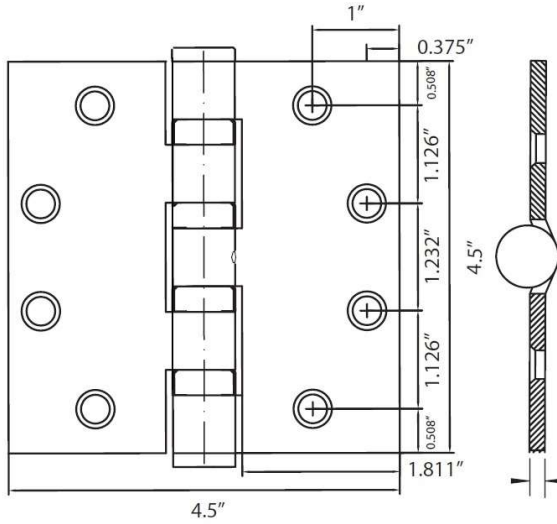
4.5" x 4.5" x SQ
