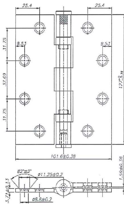
5.0" x 4.0" x SQ (127.0mm x 101.6mm)
