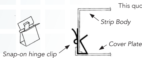
ATTACHMENT OF HINGE CLIP
