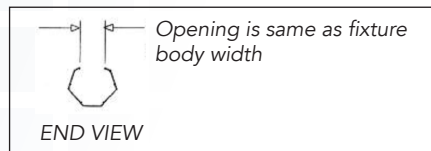
ATTACHMENT OF HINGE CLIP
