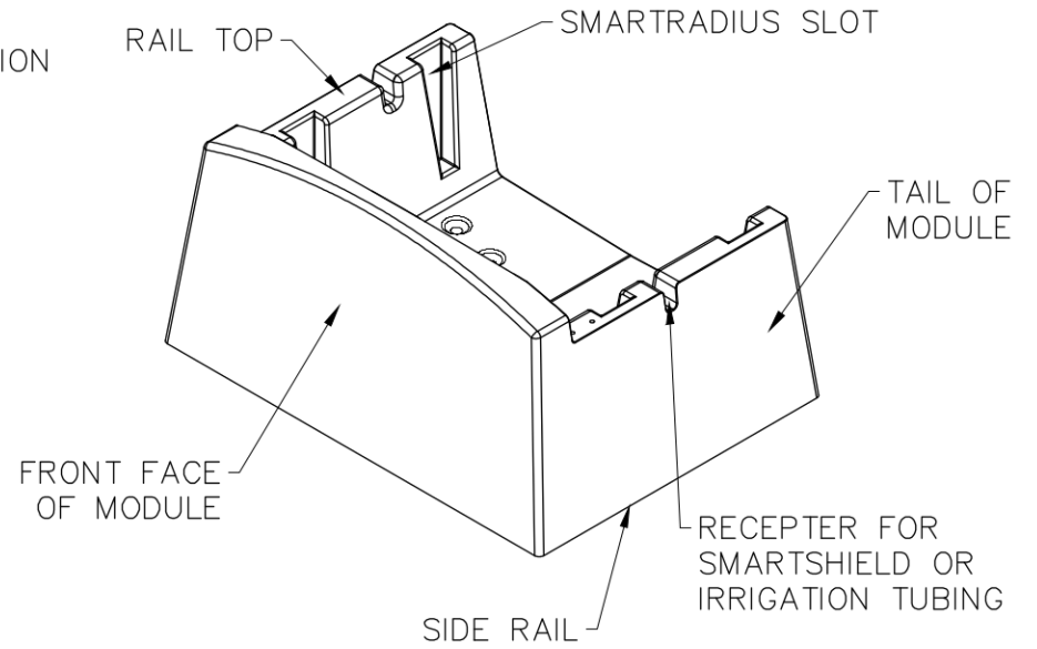
ISO VIEW
