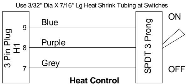
Manual Heat Control Adjust
