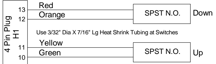
Manual Heat Control Adjust
