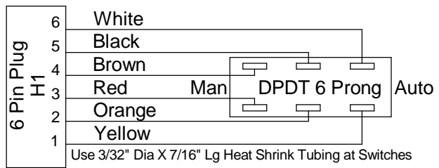
Auto / Manual Heat Control
