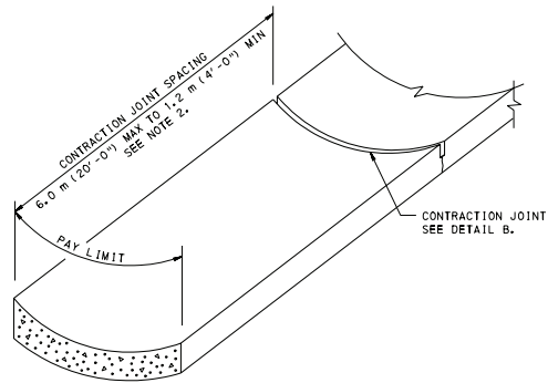
PLAIN CEMENT CONCRETE GUTTER
