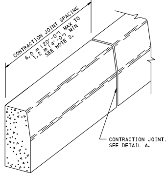
PLAIN CEMENT CONCRETE CURB
