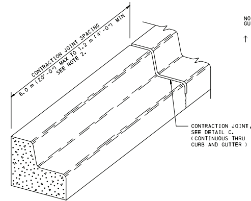
PLAIN CEMENT CONCRETE CURB GUTTER
