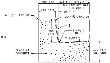
TYPICAL CROSS SECTION
