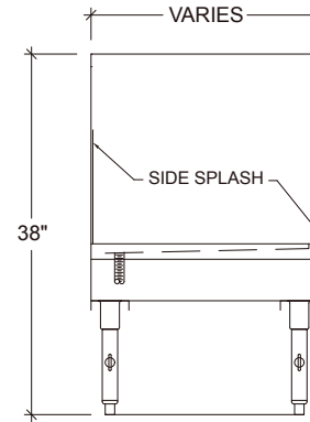
'S' or 'D' SERIES RECESSED ELEVATION
