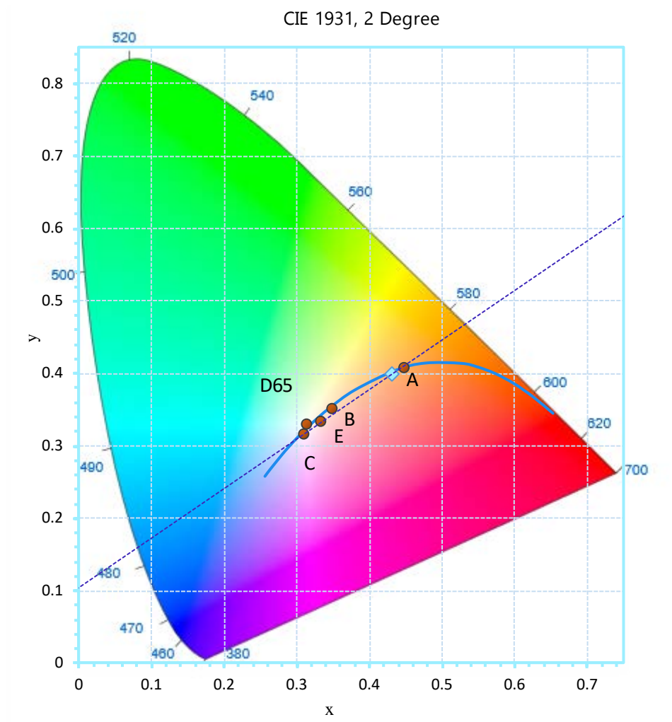
Chart 2. Chromaticity Diagram
