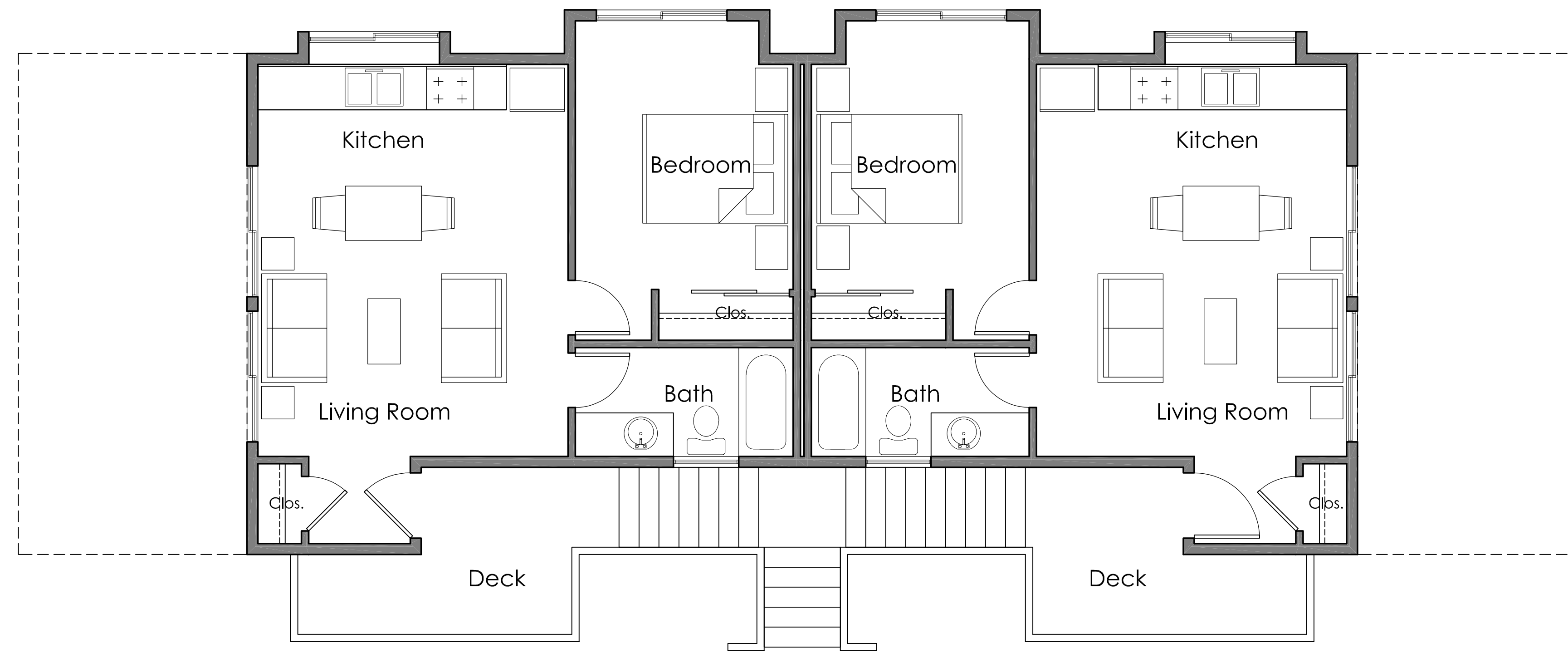
UPPER FLOOR PLAN 2 Units @ 534 sf Gross Floor Area = 1,068 sf
