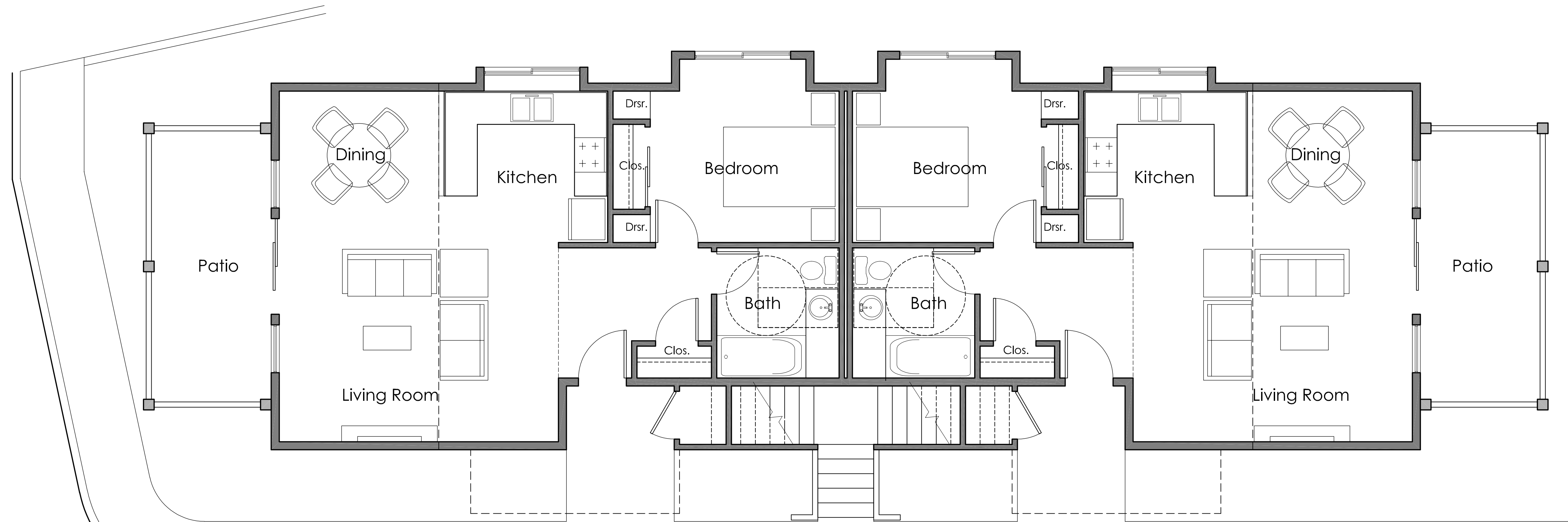
LOWER FLOOR PLAN 2 Units @ 774 sf Gross Floor Area = 1,548 sf
