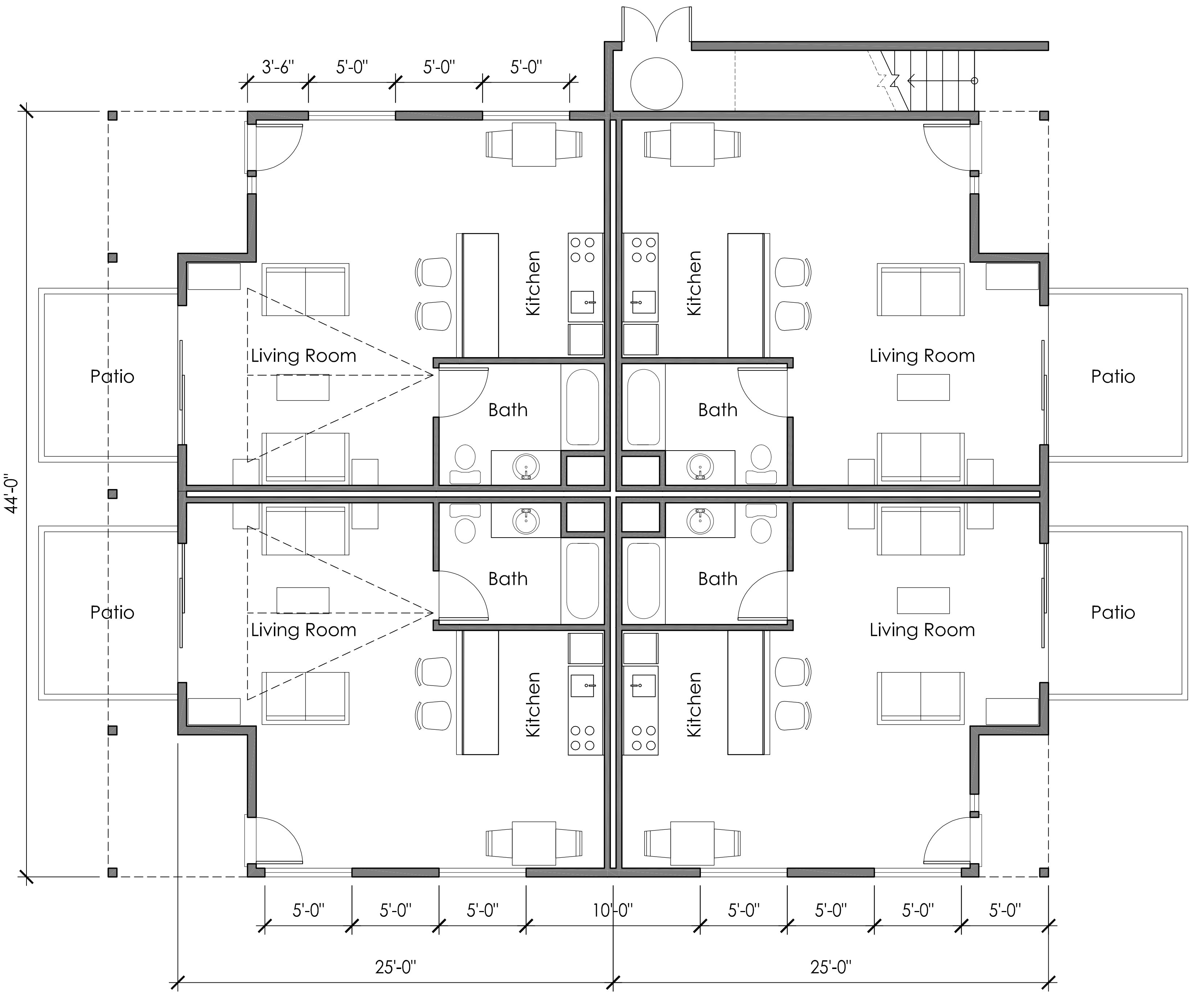
LOWER FLOOR PLAN
