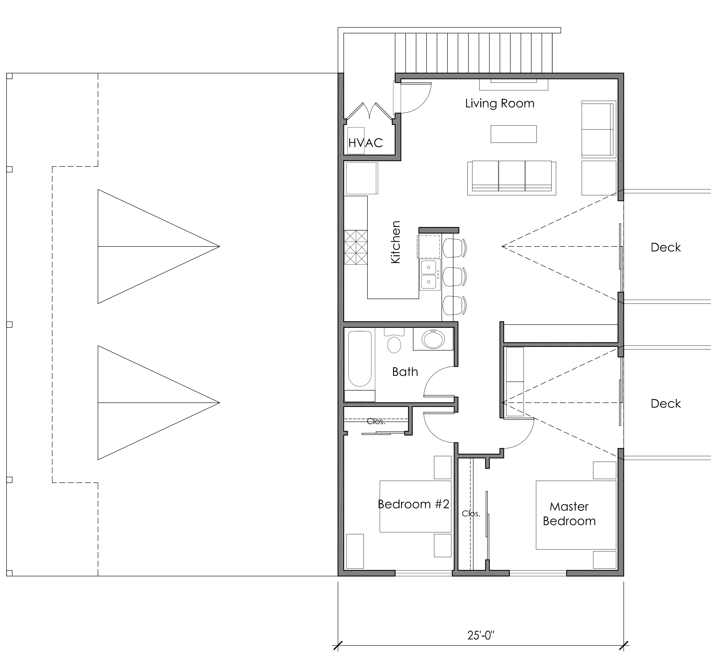
UPPER FLOOR PLAN
