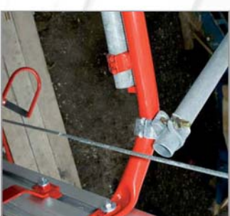
Mast fixing – The aluminium mast can be steplessly fixed to the scaffold resp. building.
