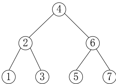
Fig. 2. Product hash value index tree
