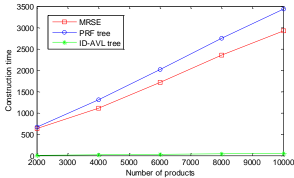
Fig. 4. Construction time of the index structures
