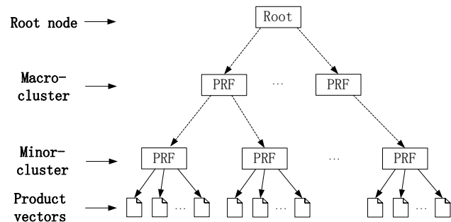
Fig. 3. Product retrieval feature tree
