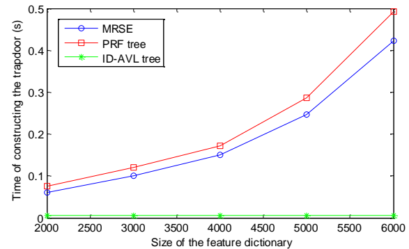
Fig. 5. Time of constructing the trapdoors
