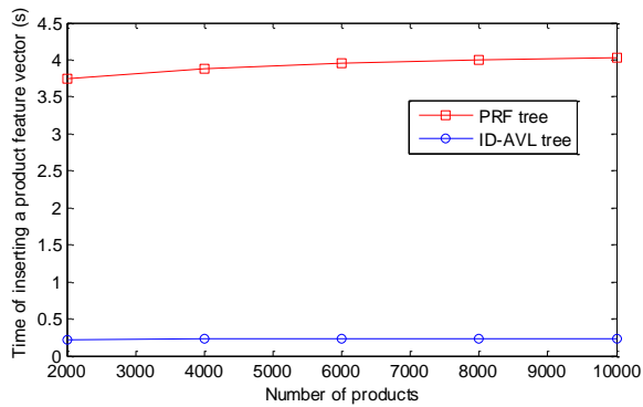
Fig. 7. Time consumption of inserting a node into the trees
