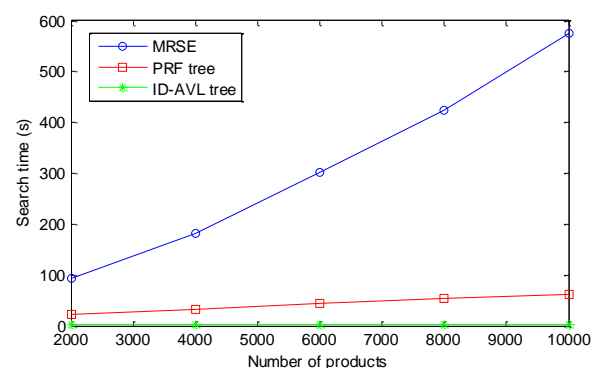
Fig. 6. Search time with different number of products
