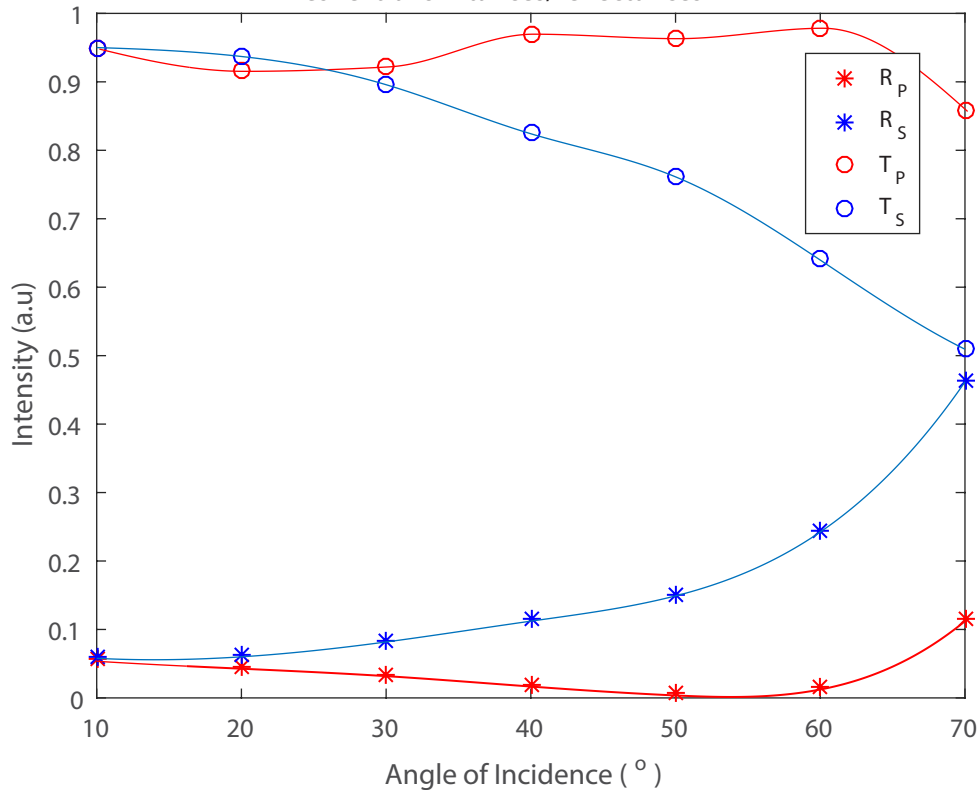
Fresnel transmittances/reflectances
