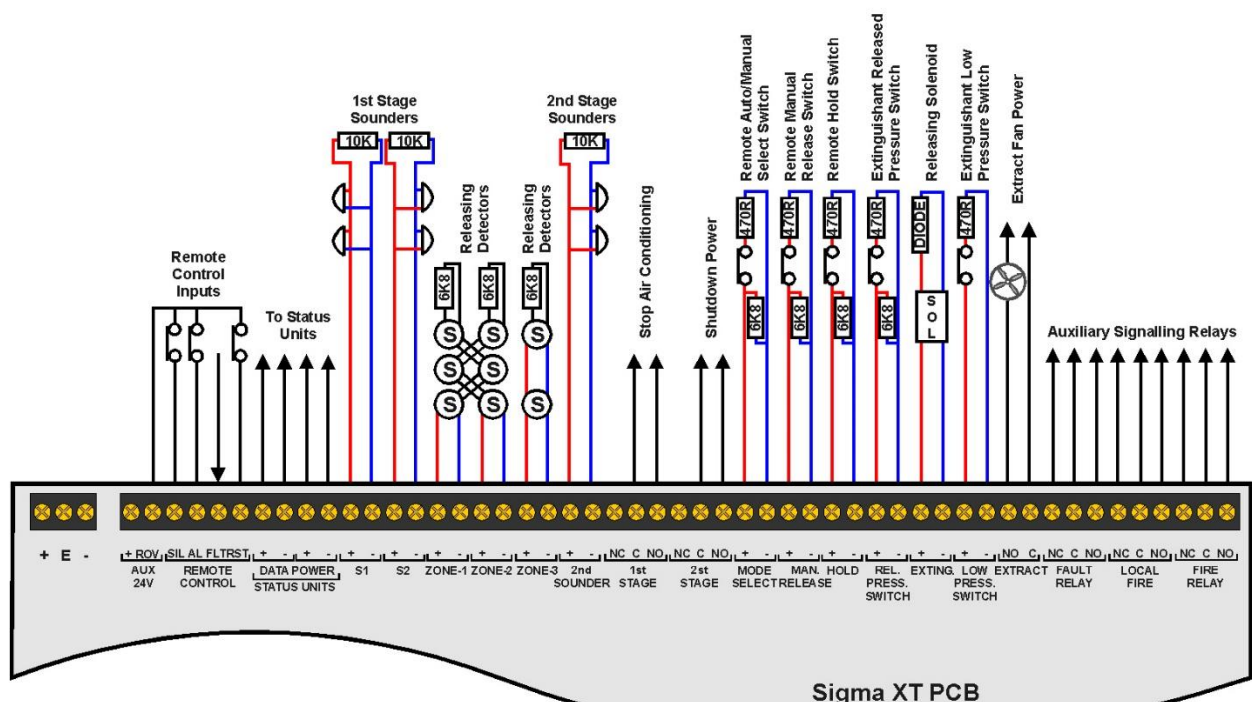
Figure 22 - System Schematic
